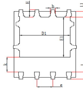
Bottom View [背视图]
